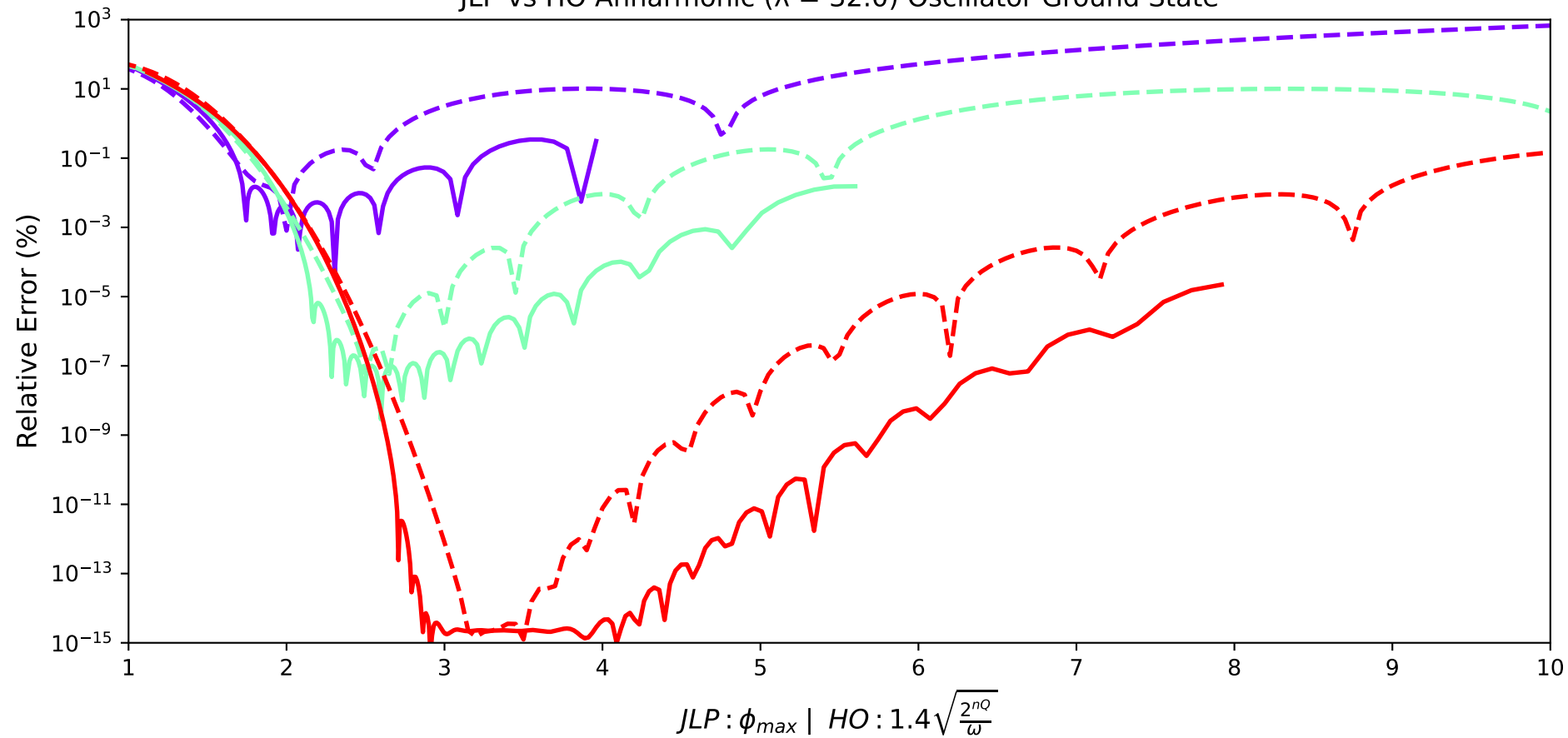
JLP vs HO Anharmonic ( \lambda = 32.0 ) Oscillator Ground State
